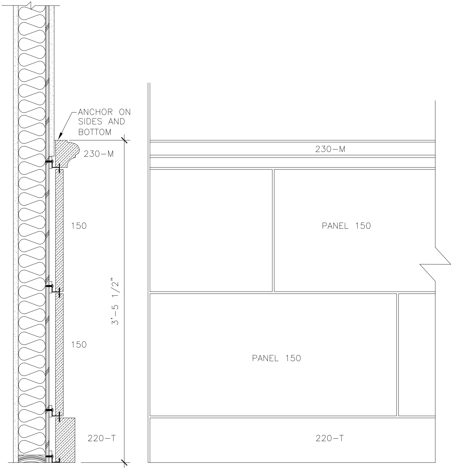
1 WAINSCOT ELEVATION & SECTION PANEL 150 AND PROFILES 230-M AND 220-T SHOWN
