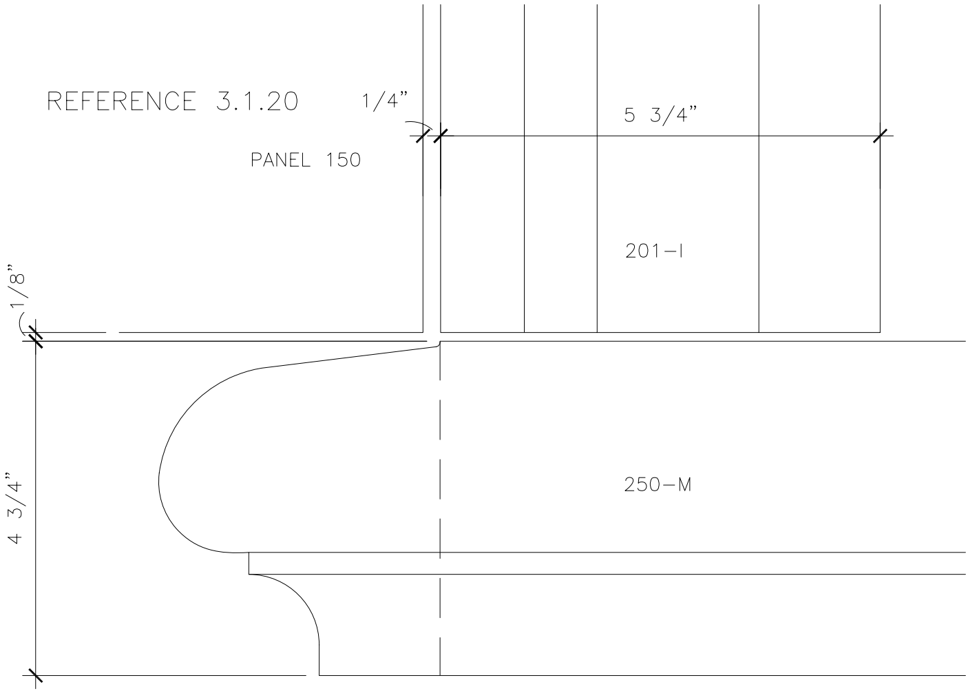
2 ELEVATION VIEW
