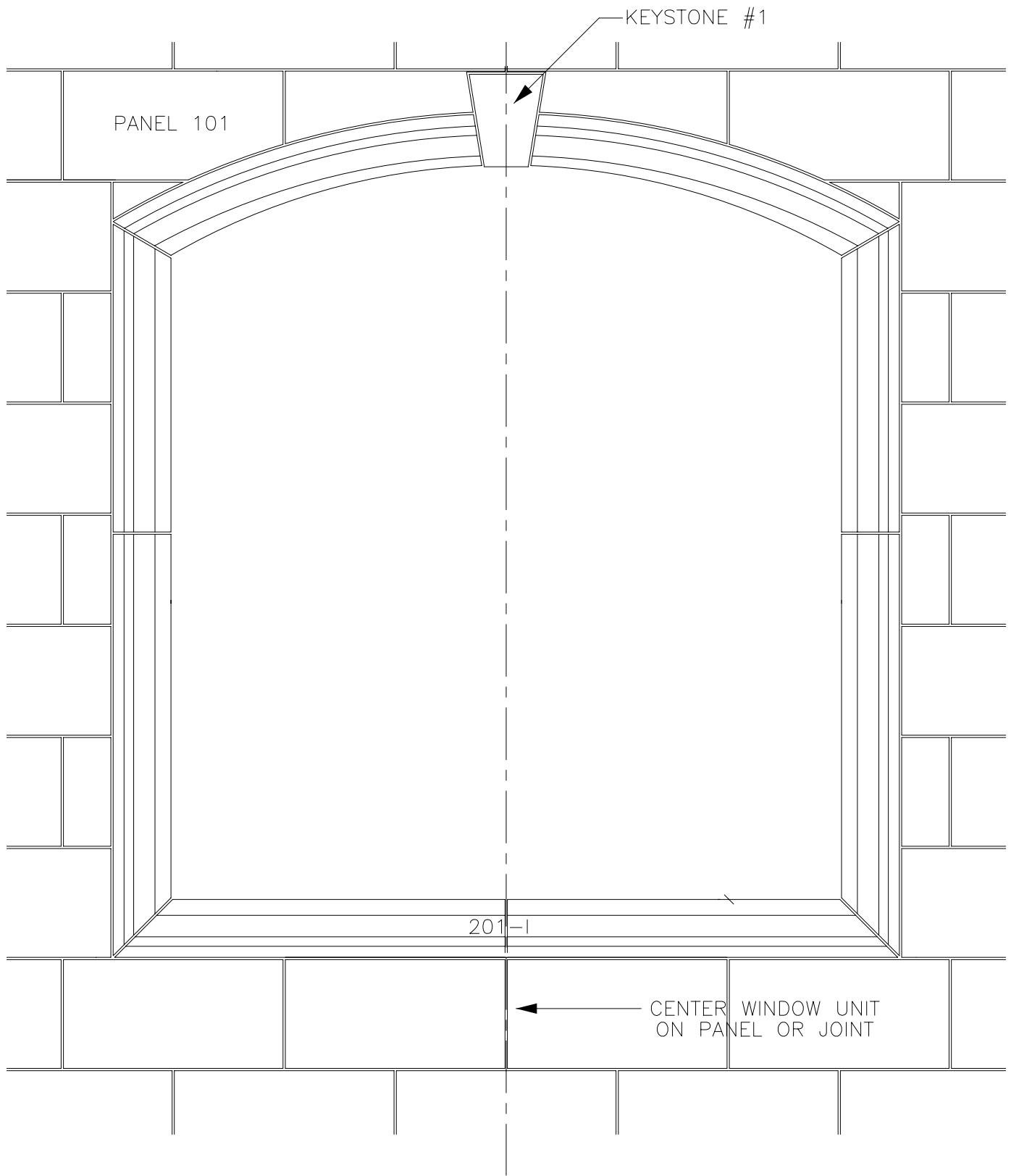
1 FLAT ARCHED WINDOW SURROUND WITH KEYSTONE 1 WITH PROFILE 201-I
