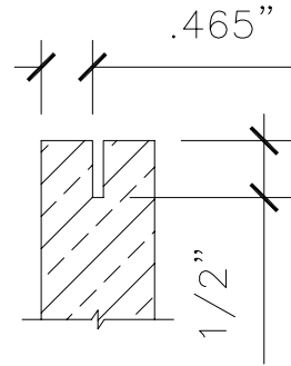
3 DETAIL-ANCHOR SLOT
